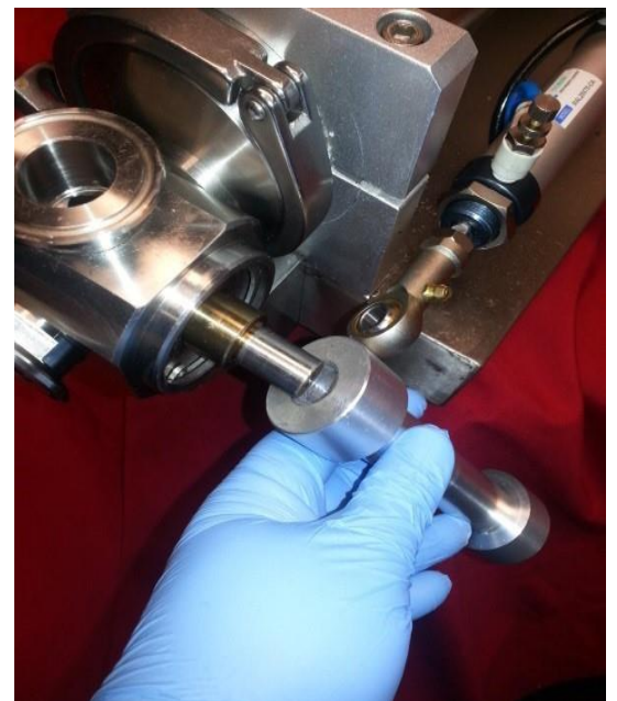
The bearing shaft driver DO NOT hit directly on the shaft us this tool
